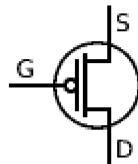
MOSFET enhanced without bulk (body terminal) shown
